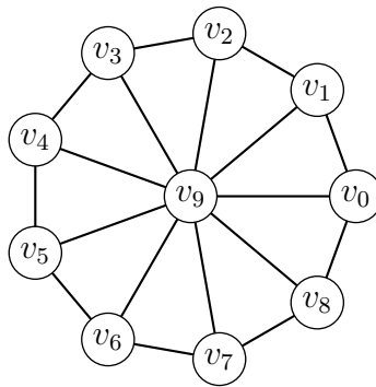
Figura 1.14: Roda W_{10}
